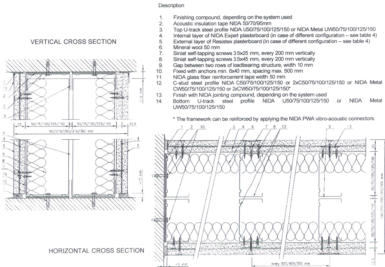
Fig. no. 4. Vertical and horizontal cross-section of anti-burglar non-loadbearing partition wall with double framework (rows of profiles separated) and two layers of boards.
